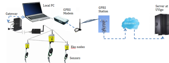
Figure 4: System Architecture.
