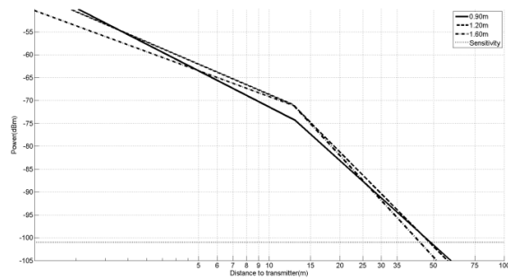
Figure 2: Propagation equations in scrublands.
