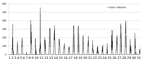
Figure 10: Solar radiation ( \text{W/m}^2 ) Node 7.
